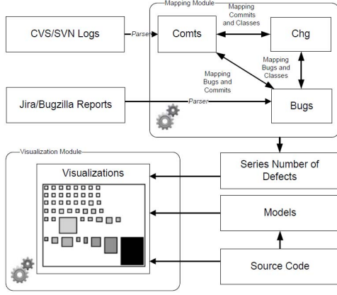
Fig. 1. BugMaps architecture
