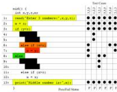
Fig. 2. Colored Code for Detecting Error Location, extracted from Jones et al. [22].
