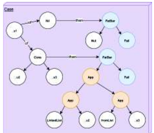
Fig. 8. Pattern Matching case Expression.
