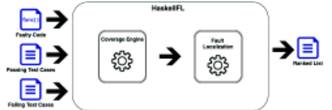
Fig. 5. HaskellFL architecture.
