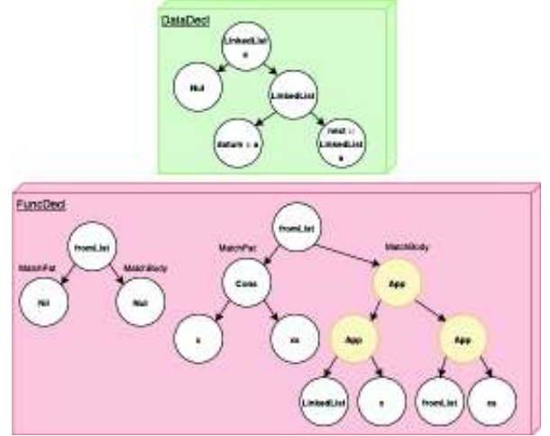
Fig. 7. LinkedList AST.
