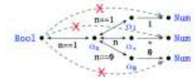
Fig. 4. Graph for Diagnosing Type Errors, extracted from Zhang et al. [50].
